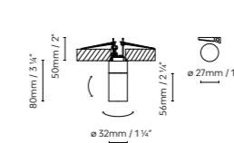
ANVIL SPOT CR SINGLE
