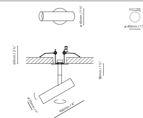
ANVIL SPOT SLIM CR
