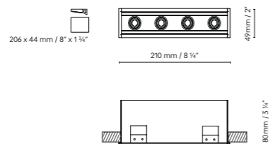
ANVIL LED MODULE R4
