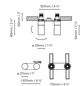
ANVIL SPOT CR DOUBLE
