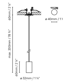
ANVIL SPOT SR
